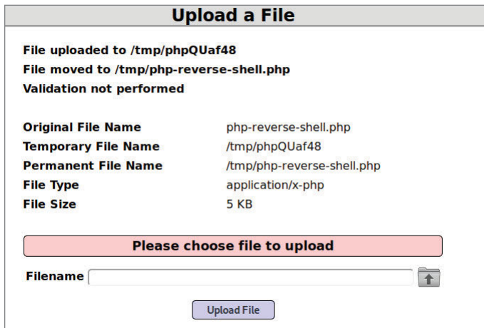
Figure 8.35: Mutillidae – File Upload Results
