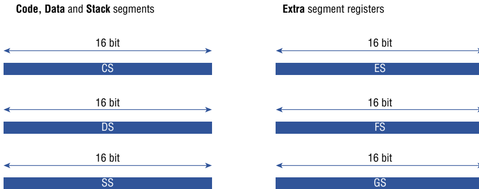
Figure 15.4: Segment Registers
